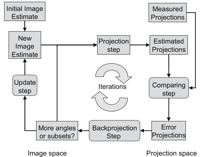
Fig. 5. The iterative procedure. The flow chart describes the steps of the iterative procedure
